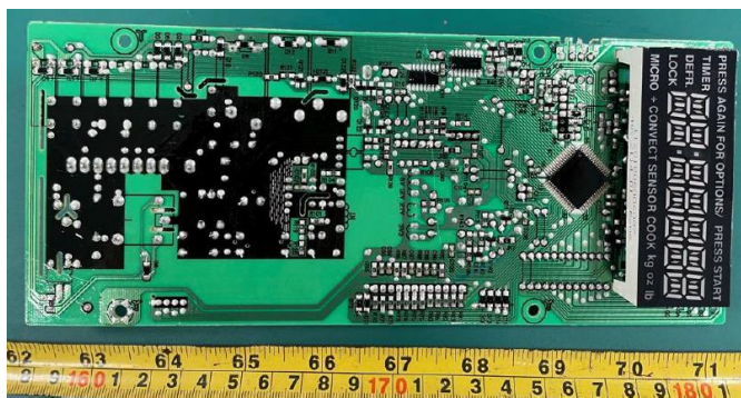
Original Mother board -bottom
