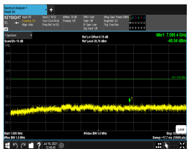
Band5-10MHz-QPSK-20600:1000~10000MHz
