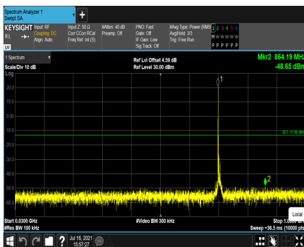
Band17-10MHz-16QAM-23800:30~1000MHz
