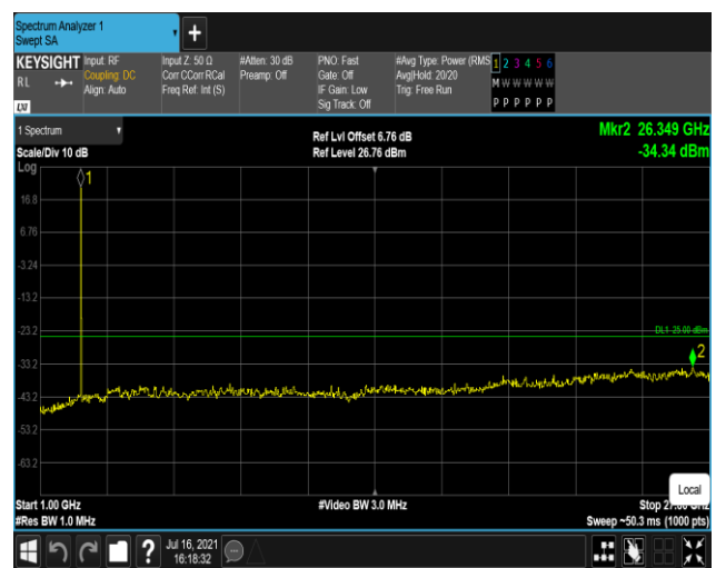
Band38-5MHz-16QAM-38225:1000~27000MHz
