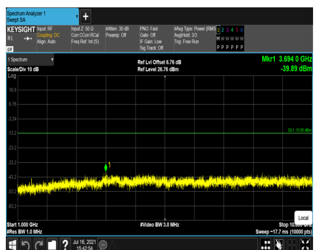
Band17-5MHz-16QAM-23825:1000~10000MHz
