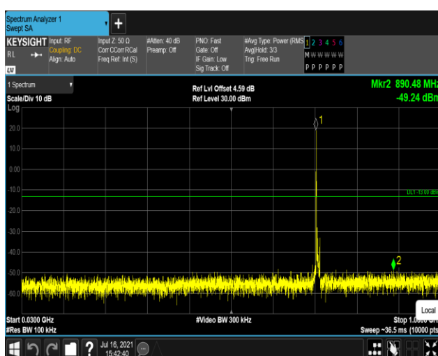
Band17-5MHz-16QAM-23825:30~1000MHz
