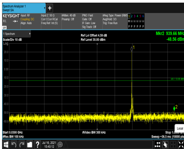
Band17-5MHz-QPSK-23790:30~1000MHz
