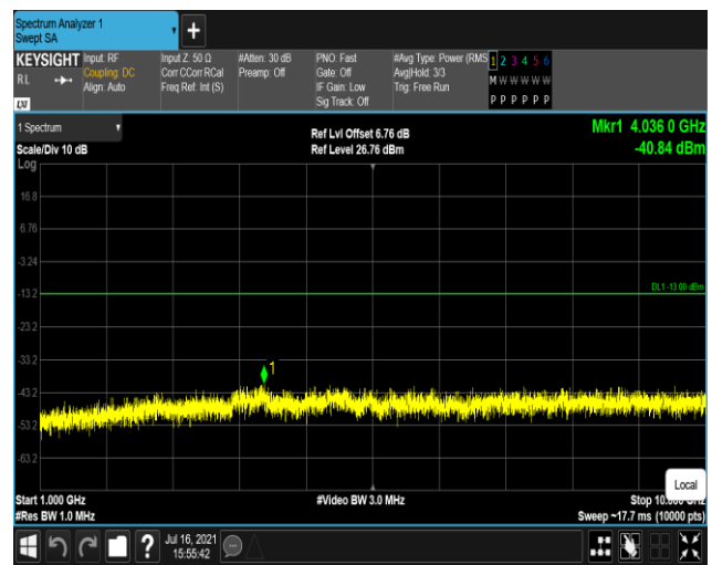
Band17-10MHz-16QAM-23790:1000~10000MHz
