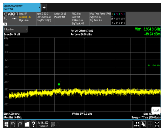
Band17-10MHz-16QAM-23800:1000~10000MHz
