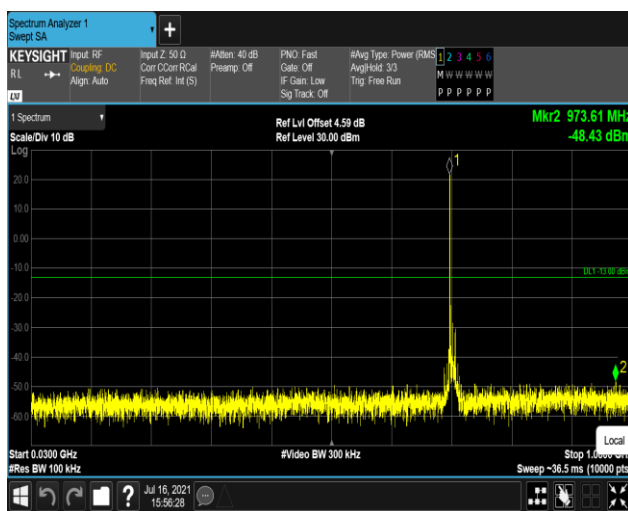
Band17-10MHz-16QAM-23800:30~1000MHz
