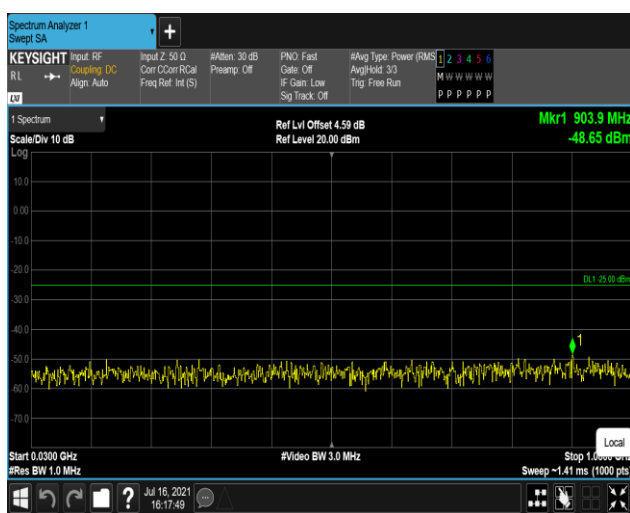
Band38-5MHz-QPSK-38225:30~1000MHz
