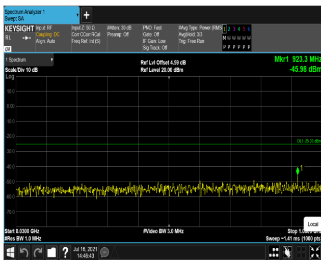
Band7-5MHz-QPSK-21425:30~1000MHz
