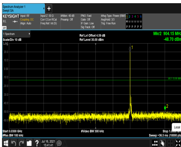
Band17-5MHz-16QAM-23825:30~1000MHz
