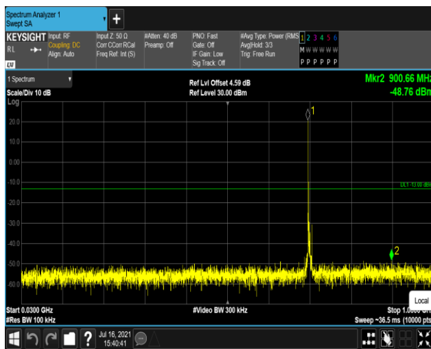
Band17-5MHz-16QAM-23790:30~1000MHz
