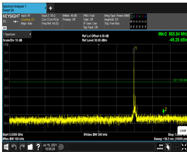
Band17-10MHz-16QAM-23790:30~1000MHz
