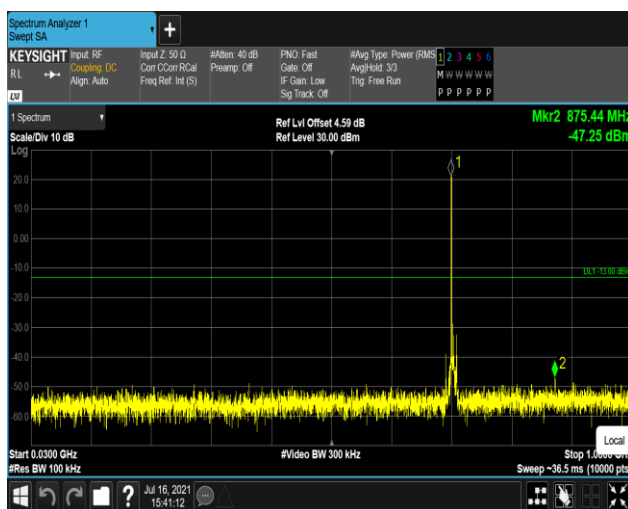
Band17-5MHz-QPSK-23825:30~1000MHz
