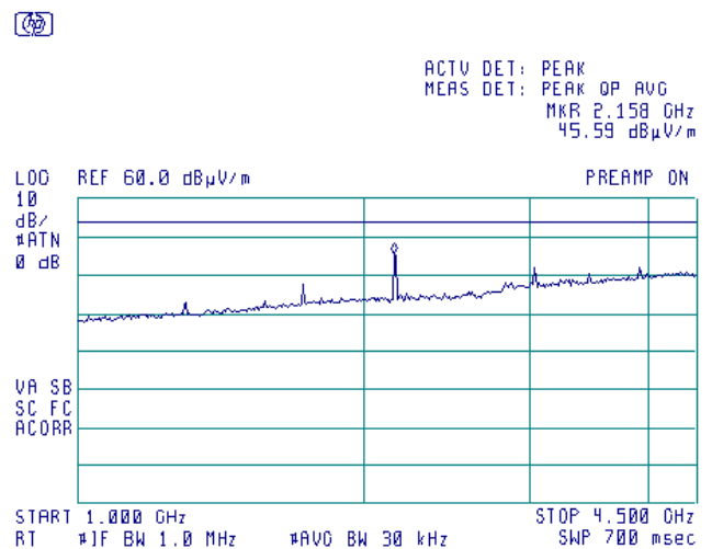
Plot 7.2.17 Radiated emission measurements from 1000 to 4500 MHz at mid frequency
