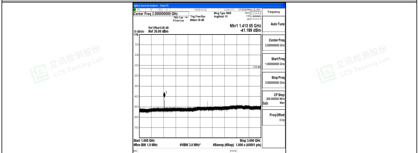
Band12_10MHz_16QAM_23130_1RB#0_1000~3000_1000~3000
