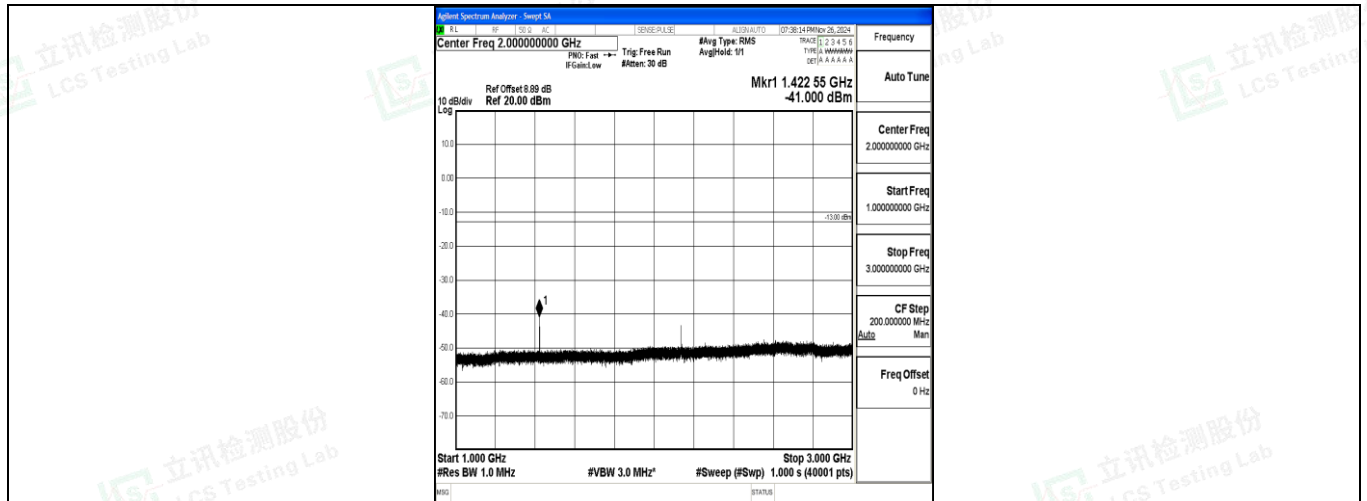
Band12_5MHz_QPSK_23155_1RB#0_1000~3000_1000~3000
