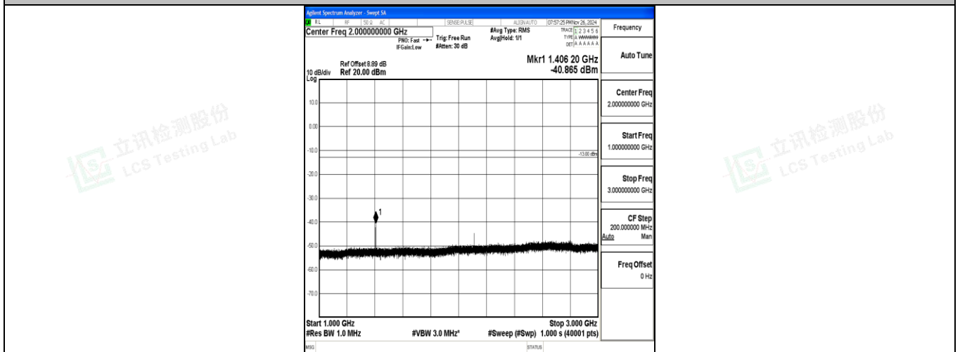
Band12_10MHz_QPSK_23095_1RB#0_1000~3000_1000~3000
