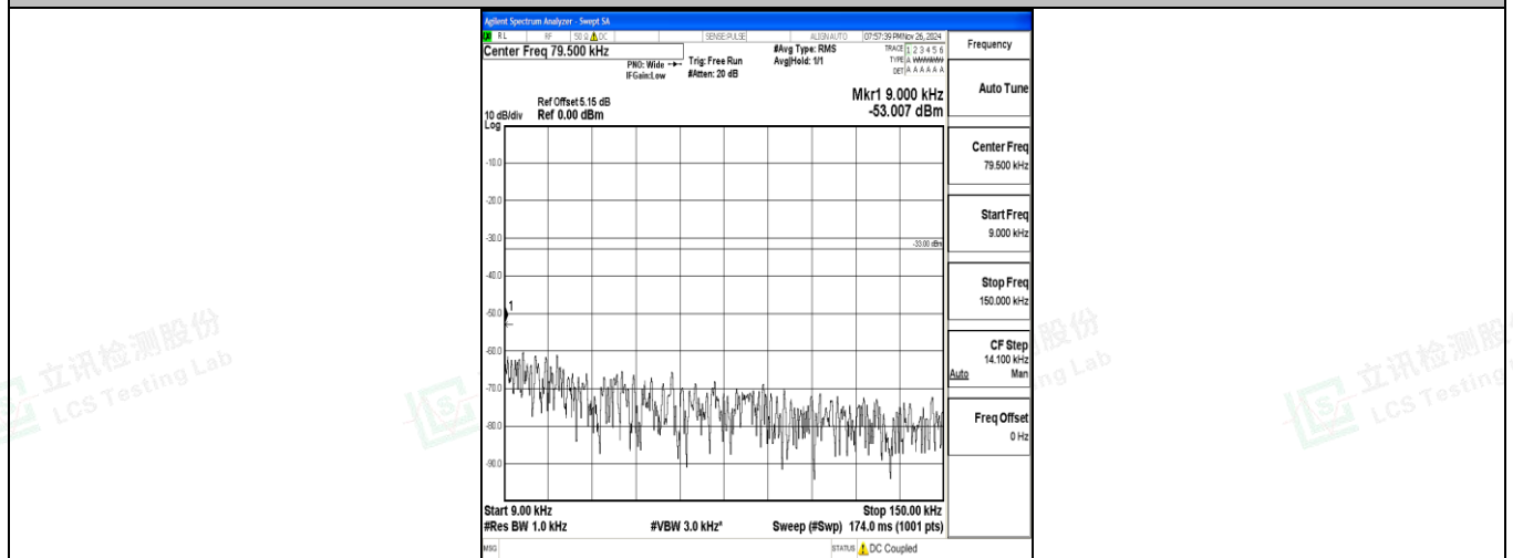
Band12_10MHz_16QAM_23095_1RB#0_0.009~0.15_0.009~0.15
