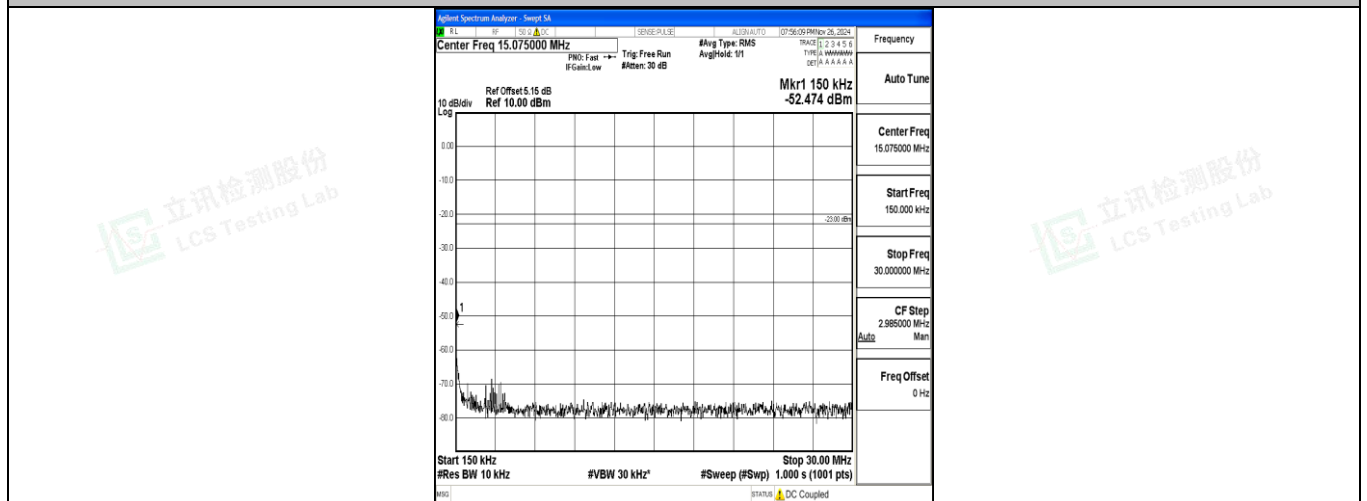
Band12_10MHz_QPSK_23060_1RB#0_0.15~30_0.15~30
