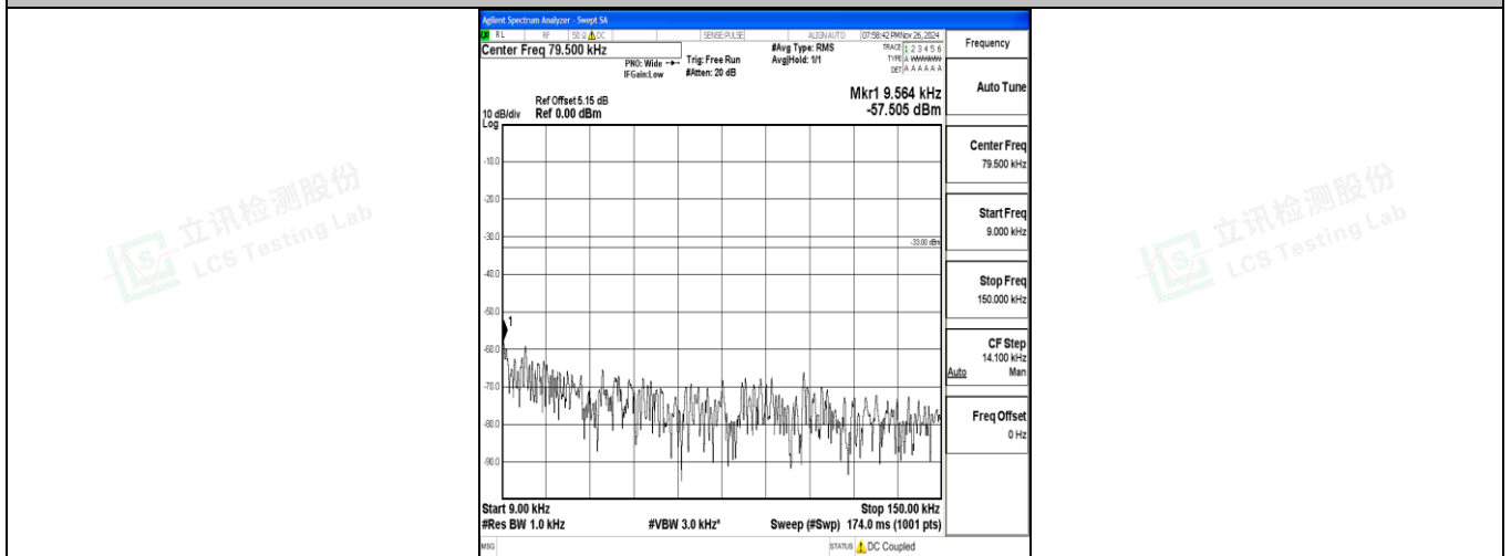
Band12_10MHz_16QAM_23130_1RB#0_0.009~0.15_0.009~0.15
