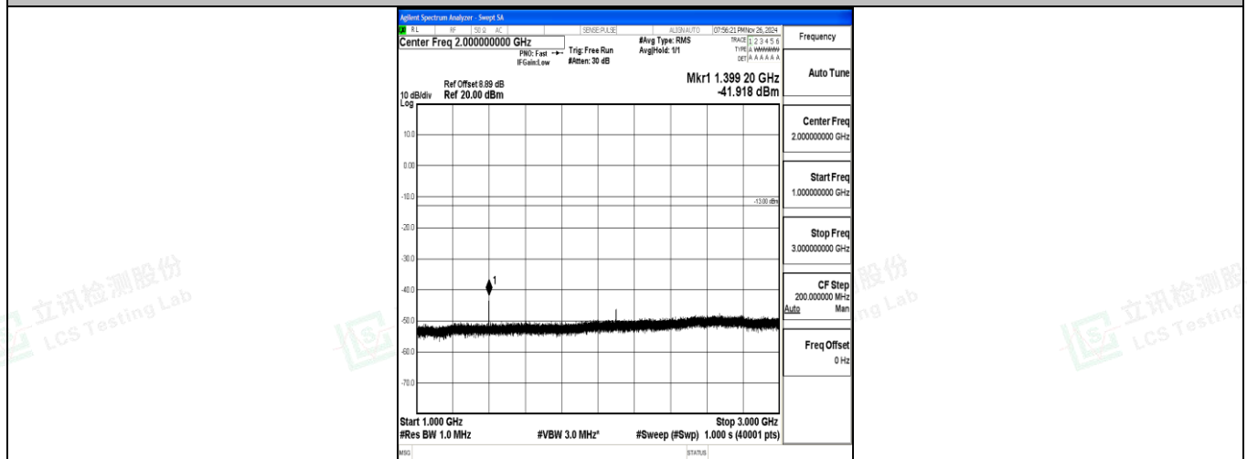
Band12_10MHz_QPSK_23060_1RB#0_1000~3000_1000~3000
