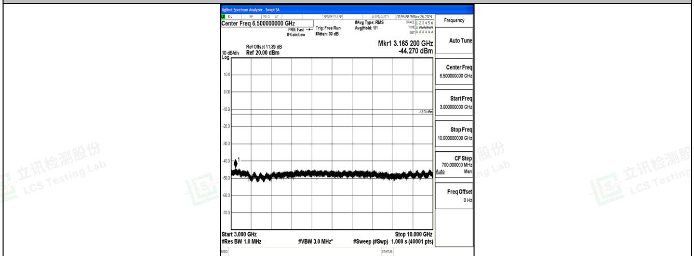
Band12_10MHz_16QAM_23060_1RB#0_3000~10000_3000~10000
