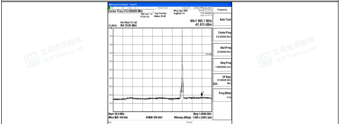
Band12_10MHz_QPSK_23130_1RB#0_30~1000_30~1000
