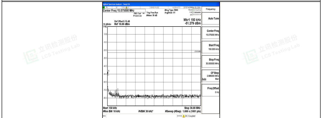
Band12_10MHz_16QAM_23095_1RB#0_0.15~30_0.15~30
