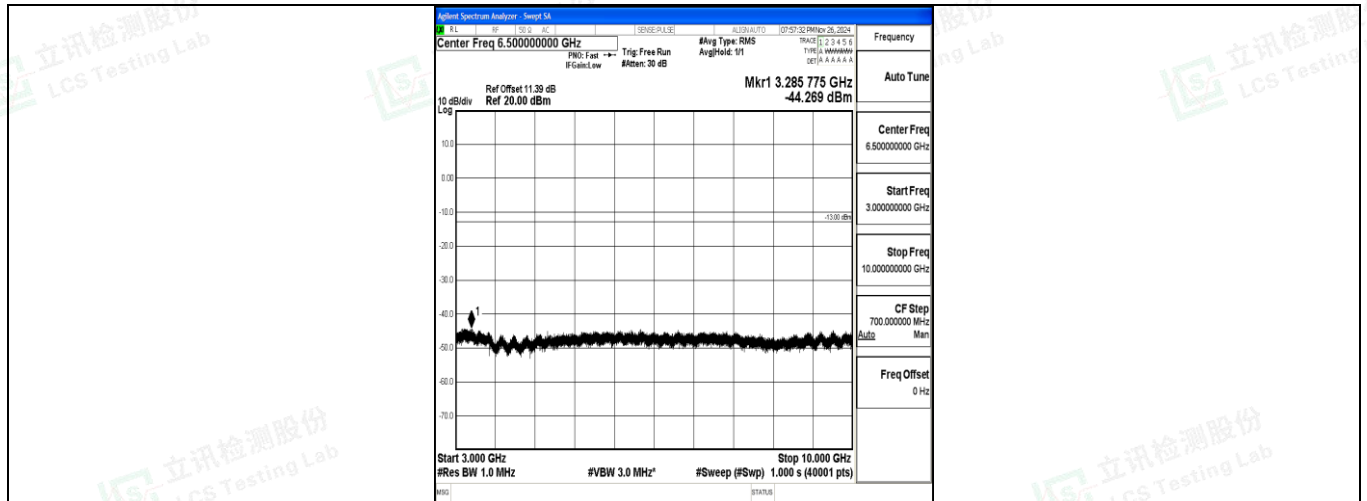
Band12_10MHz_QPSK_23095_1RB#0_3000~10000_3000~10000
