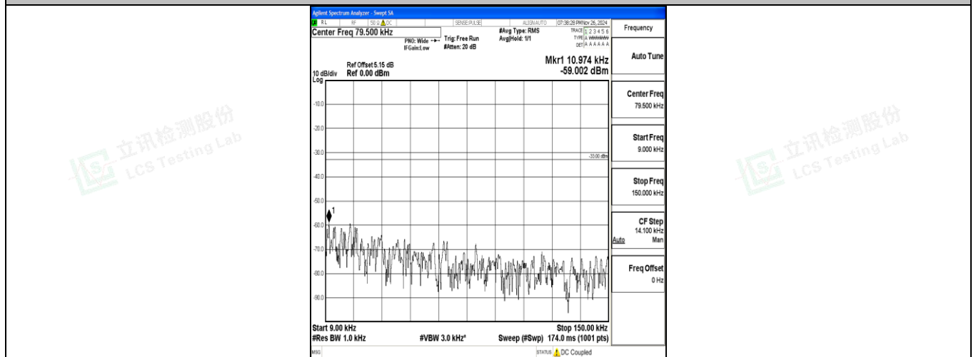
Band12_5MHz_16QAM_23155_1RB#0_0.009~0.15_0.009~0.15
