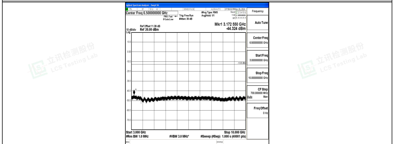
Band12_10MHz_16QAM_23095_1RB#0_3000~10000_3000~10000
