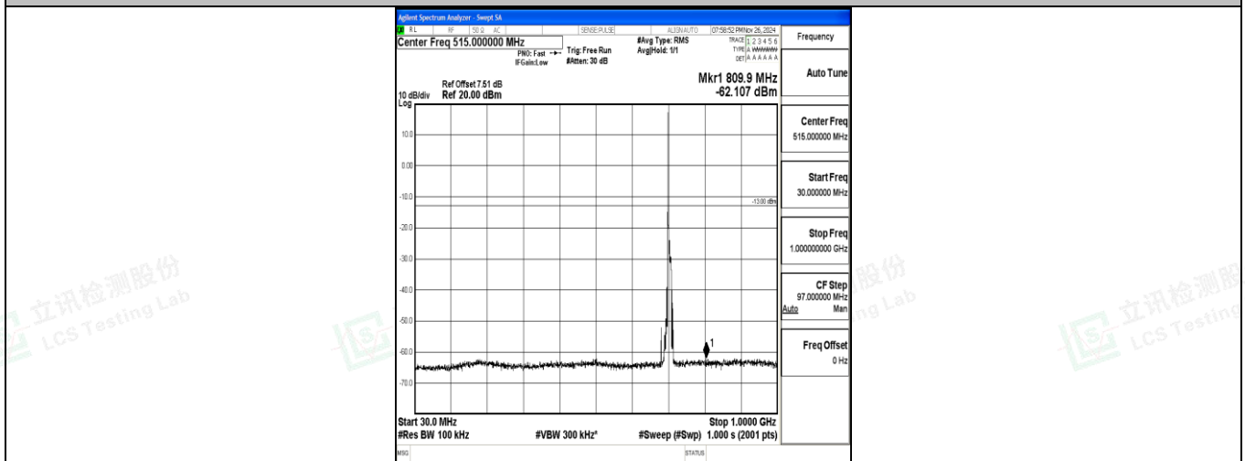
Band12_10MHz_16QAM_23130_1RB#0_30~1000_30~1000
