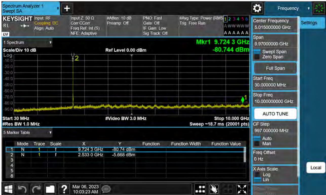
Sub6 n7. Conducted Spurious_1 (507000ch_5 MHz_BPSK_RB 1)
