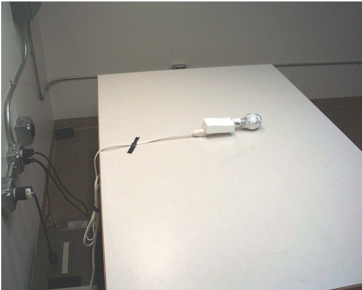
Back View Conducted Disturbance Worst Case Configuration
