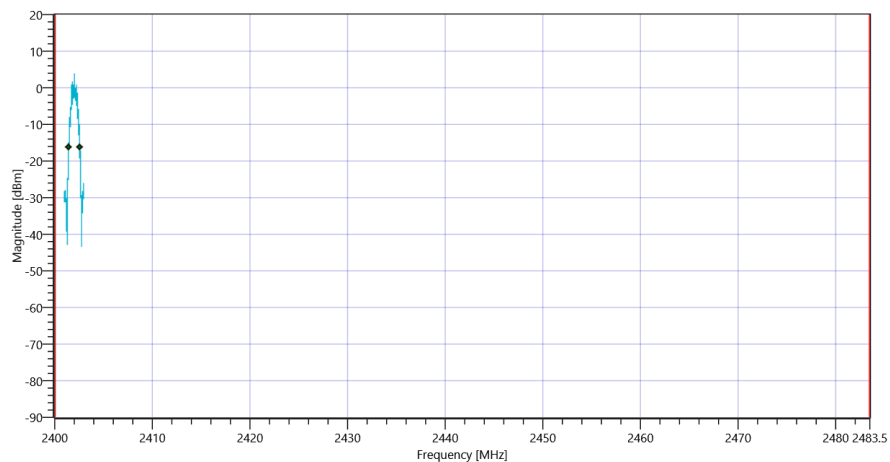
Plot_FCC Part 15.247 Bandwidth 99PCT-20dB ~ BT LE 1 Msps_29072019_102625.png
