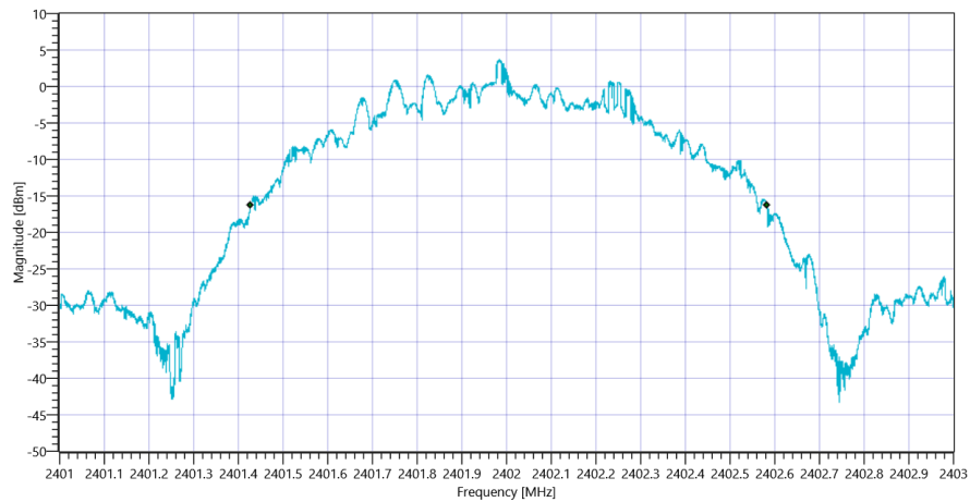
Plot_FCC Part 15.247 Bandwidth 99PCT-20dB ~ BT LE 1 Msps_29072019_102622.png
