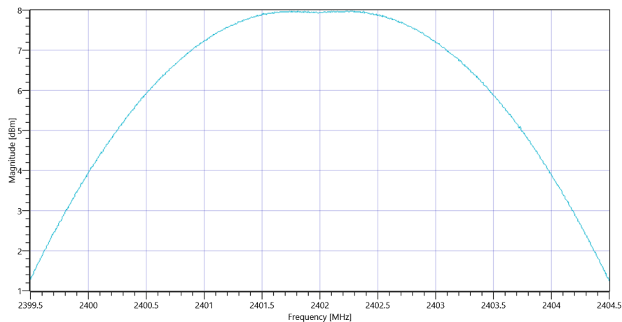
Plot_Common2G4 Peak Output Power conducted 3MHz_3MHz ~ BT LE 1 Msps_29072019_130523.png
