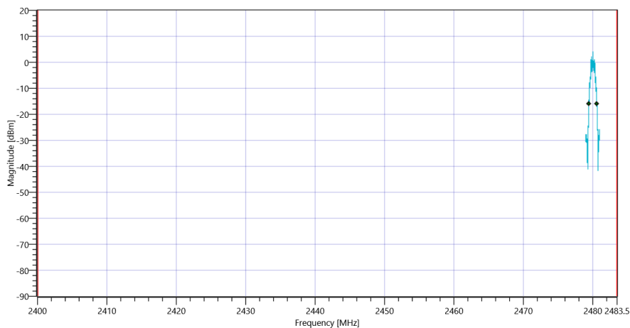
Plot_FCC Part 15.247 Bandwidth 99PCT-20dB ~ BT LE 1 Msps_29072019_102808.png
