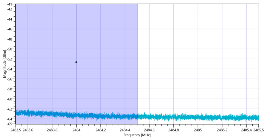
Plot_FCC Part 15.247 Restricted Band Edge Conducted Avg DC corrected DTS ~ BT LE 1 Msps_29072019_104621.png
