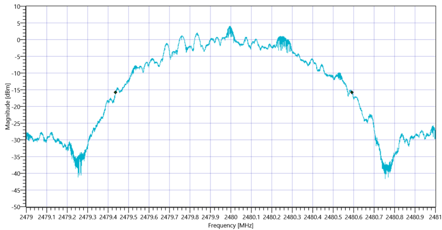
Plot_FCC Part 15.247 Bandwidth 99PCT-20dB ~ BT LE 1 Msps_29072019_102805.png
