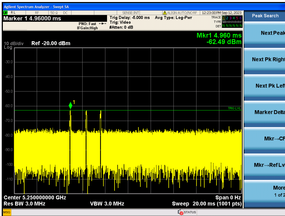
Radar Signal 5
