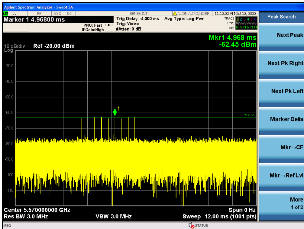
Radar Signal 6
