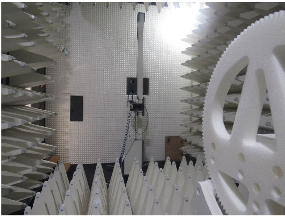
Testsetup above 1 GHz
