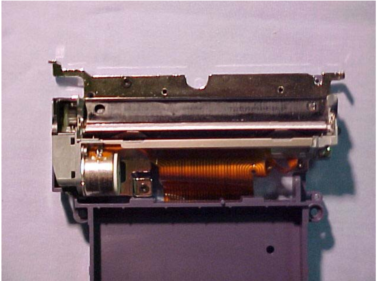
Paper Feed and Motor
