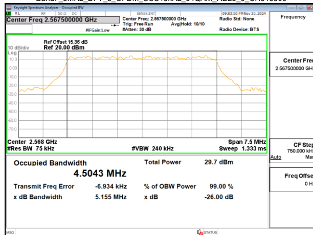
Band7_5MHz_DFT_s_OFDM_SCS15kHz_64QAM_RB25_0_CH513500
