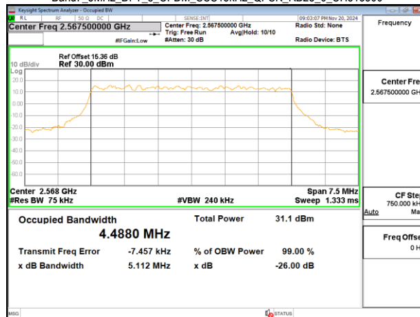
Band7_5MHz_DFT_s_OFDM_SCS15kHz_QPSK_RB25_0_CH513500
