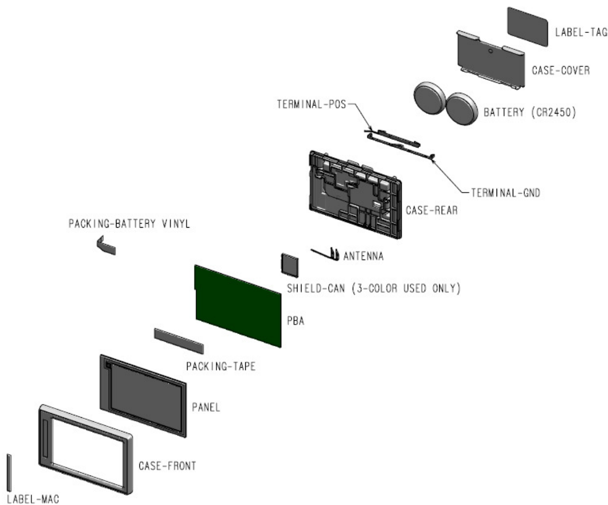
Figure 4 Exploded View
