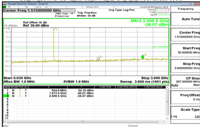
Cat_M1_30MHz~3GHz_Band5_5MHz_QPSK_1_0_MidCH20525-836.5
