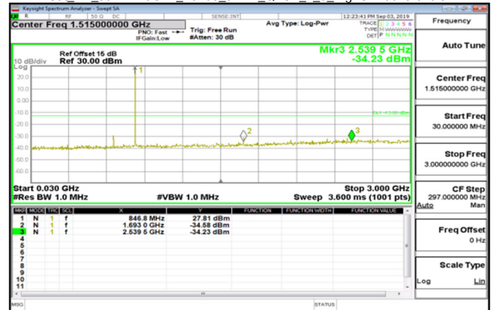
Cat_M1_30MHz~3GHz_Band5_5MHz_QPSK_1_0_HighCH20625-846.5
