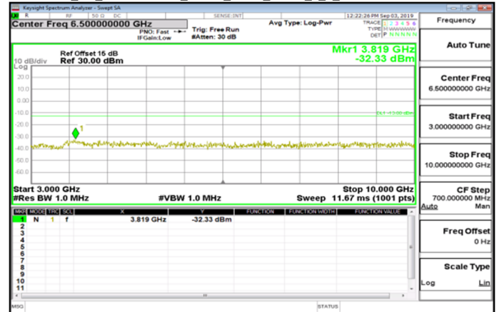
Cat_M1_3GHz~10GHz_Band5_5MHz_QPSK_1_0_MidCH20525-836.5
