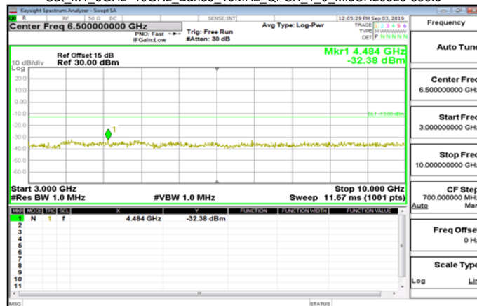
Cat_M1_3GHz~10GHz_Band5_10MHz_QPSK_1_0_MidCH20525-836.5
