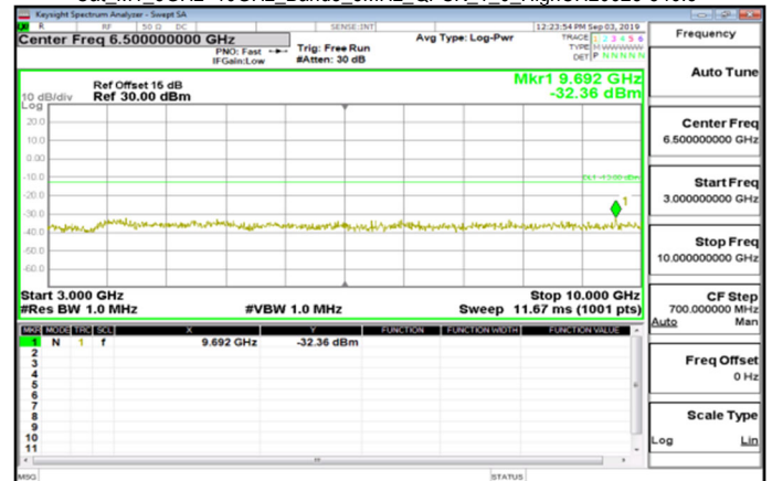
Cat_M1_3GHz~10GHz_Band5_5MHz_QPSK_1_0_HighCH20625-846.5
