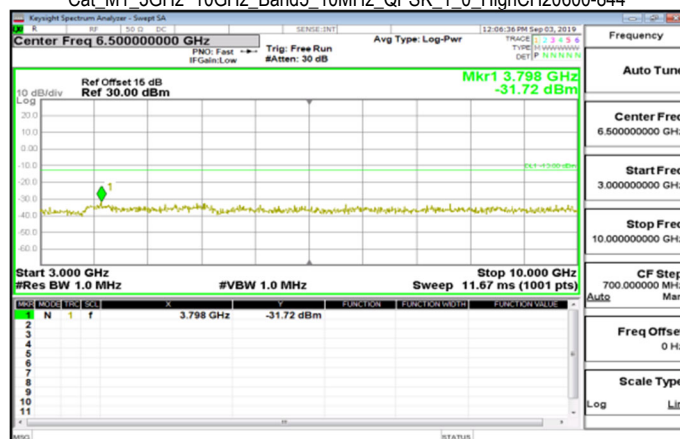
Cat_M1_3GHz~10GHz_Band5_10MHz_QPSK_1_0_HighCH20600-844
