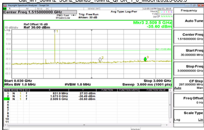
Cat_M1_30MHz~3GHz_Band5_10MHz_QPSK_1_0_MidCH20525-836.5
