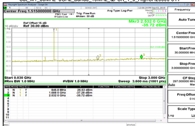
Cat_M1_30MHz~3GHz_Band5_10MHz_QPSK_1_0_HighCH20600-844
