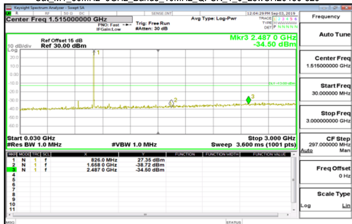
Cat_M1_30MHz~3GHz_Band5_10MHz_QPSK_1_0_LowCH20450-829
