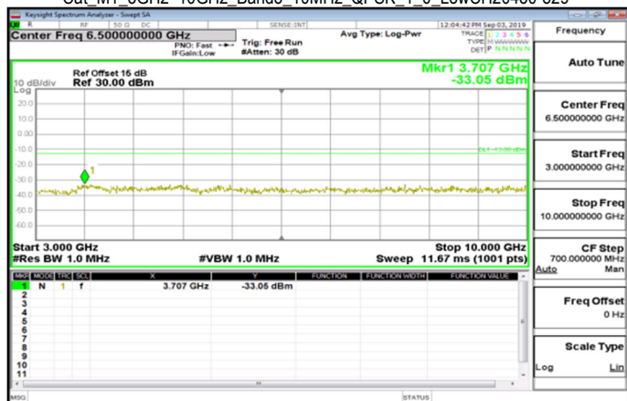
Cat_M1_3GHz~10GHz_Band5_10MHz_QPSK_1_0_LowCH20450-829
