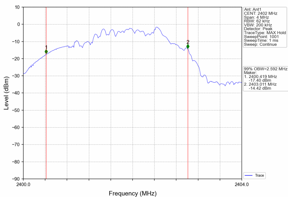
2M_LCH_2402MHz_Ant1_NTNV
