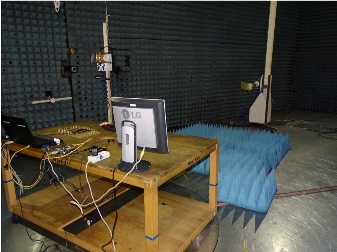
Photo 4: Test setup for radiated measurements (computer peripheral setup, EUT supplied by USB-cable from computer, unintentional radiator §15.109, ANSI C63.4) Above 1GHz
