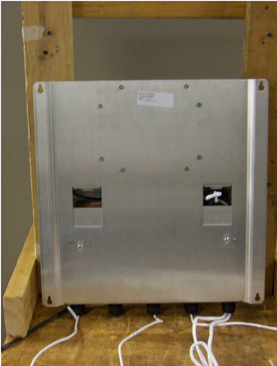
Liberty FX: Power Supply and TR4024 Control Module – Rear View
