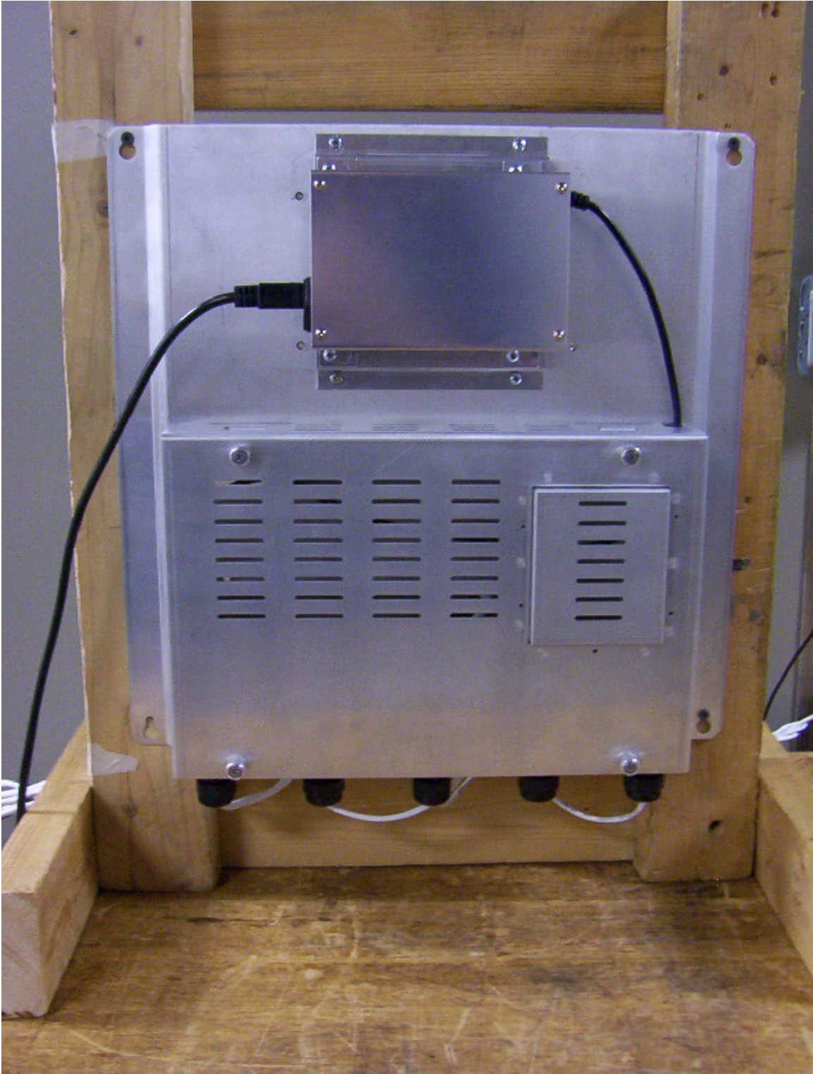
Liberty FX: Power Supply and TR4024 Control Module – Front View
