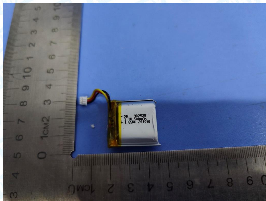
Photo 12 Battery Appearance
