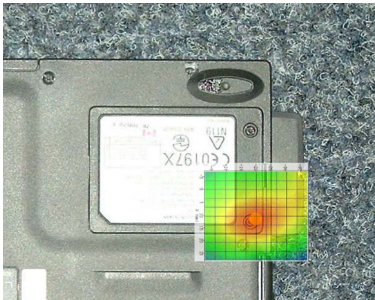
Photo 6: A 2d scan overlay giving the field strength in the first scanned plane, overlaid on a bottom side view photo of the laptop. 2d scan is that of the worst case lapheld value in channel 6.
