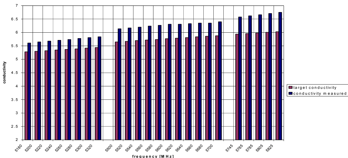
5 GHz body liquid validation
