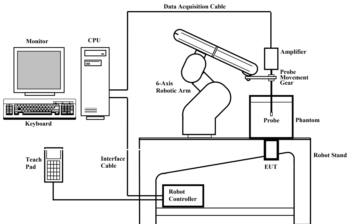
Figure 1: Overview of the SARA2 measurement system
