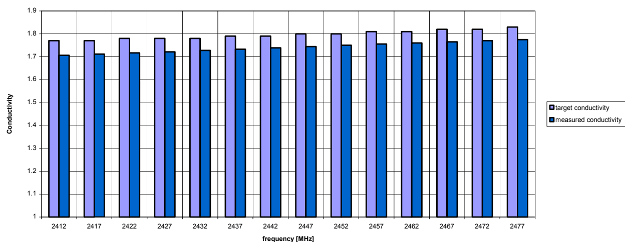
2.4 GHz head liquid validation
