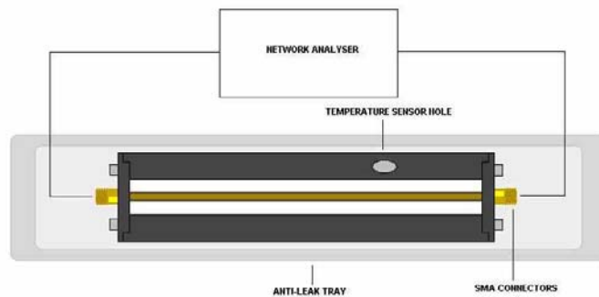
Figure 10.3.1. TEM Cell Construction.
