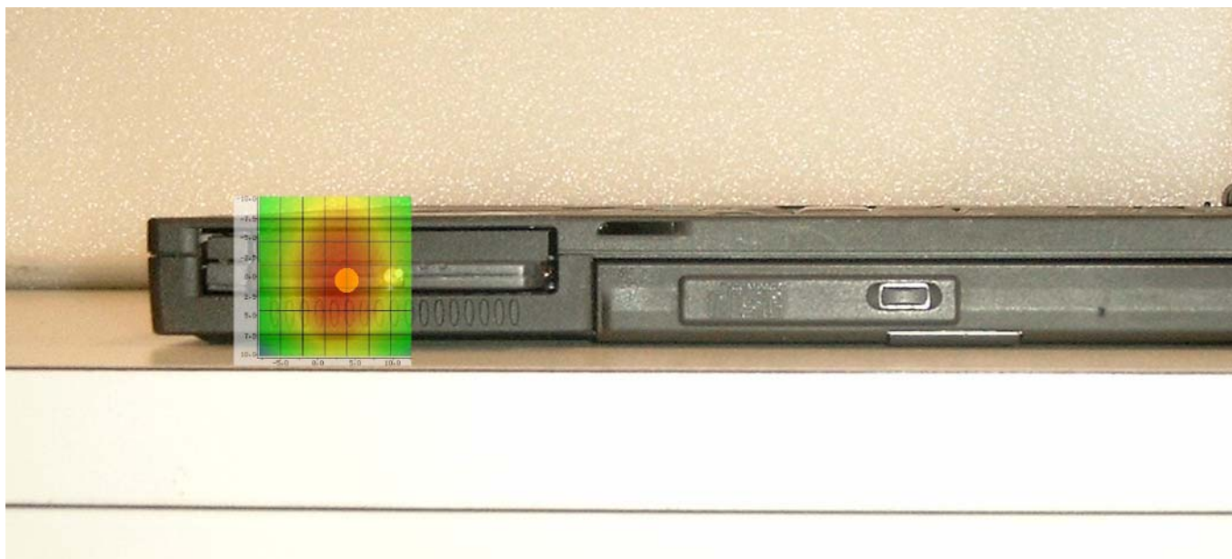
Photo 7 A 2d scan giving the field strength in the first scanned plane, overlaid on a bottom view photo of the laptop. Overlaid plot is that of the worst case perpendicular scan in channel 64
