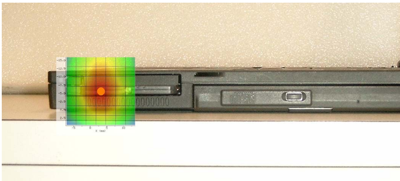
Photo 6: A 2d scan overlay giving the field strength in the first scanned plane, overlaid on a side view photo of the laptop. 2d scan is that of the worst case perpendicular value in channel 147.
