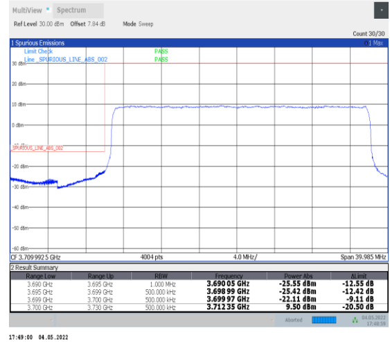
1-N78-3700-3800--30-30-L-3-DFT-PI2BPSK-Outer_Full-75@0-Ant0-PASS-see graph
