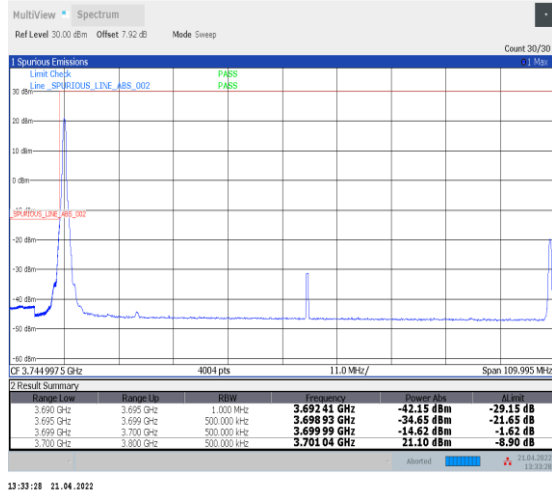
1-N78-3700-3800--30-100-L-1-DFT-PI2BPSK-Edge_1 RB_Left-1@0-Ant0-PASS-see graph
