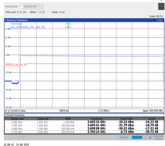
1-N78-3700-3800--30-100-L-6-CP-QPSK-Outer_F ull-273@0-Ant0-PASS-see graph
