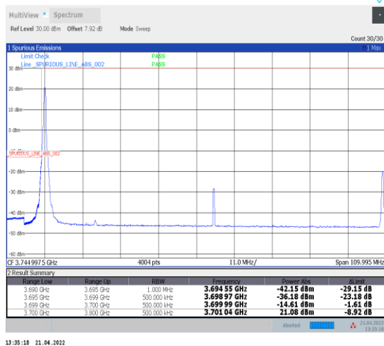
1-N78-3700-3800--30-100-L-4-CP-QPSK-Edge_1RB_ Left-1@0-Ant0-PASS-see graph
