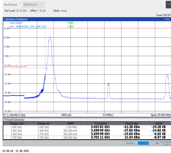
1-N78-3700-3800--30-30-L-1-DFT-PI2BPSK-Edge_1R_B_Left-1@0-Ant0-PASS-see graph
