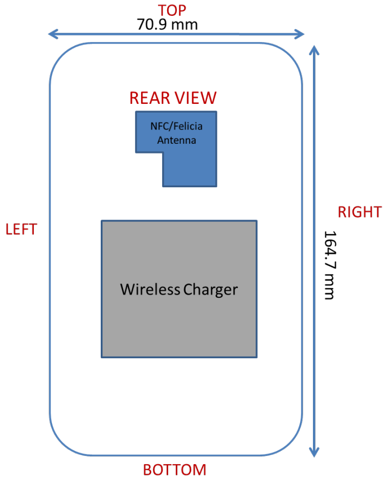
Figure J-2 NFC Antenna Locations
